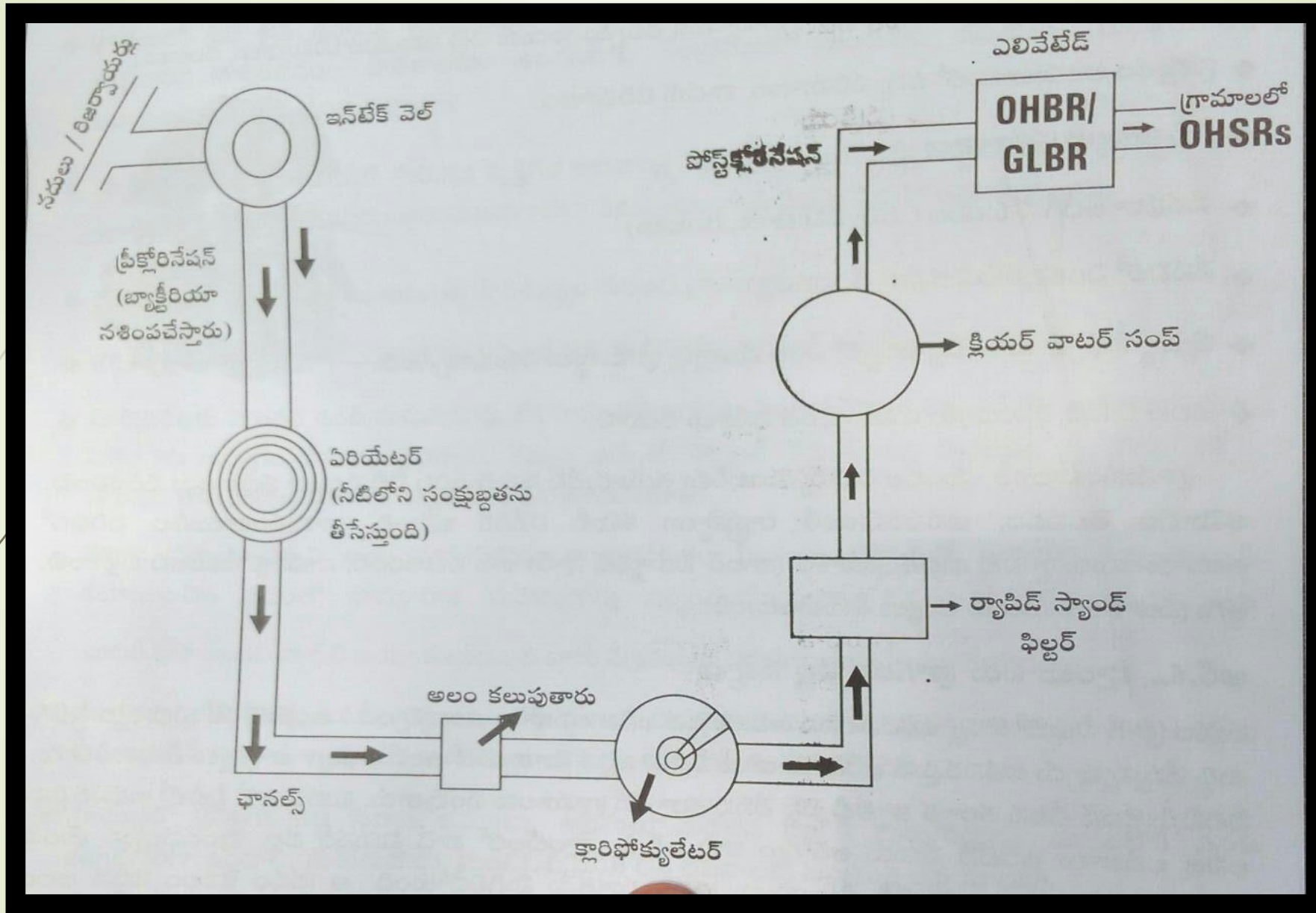
Technical Process for providing Purifying Water under Bhagiratha Mission
